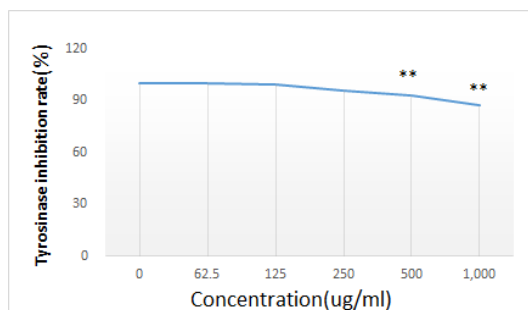
Fig. 5. The Inhibitory Effects of GE on Tyrosinase Activity in vitro. The number indicated on the X axis is the concentration of GE.
